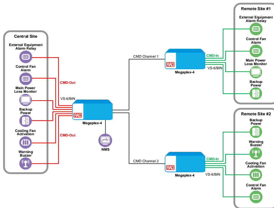
Figure 2. Input/Output Binary Relay Commands in a Point-to-Multipoint Deployment of a VS-6/BIN Module
