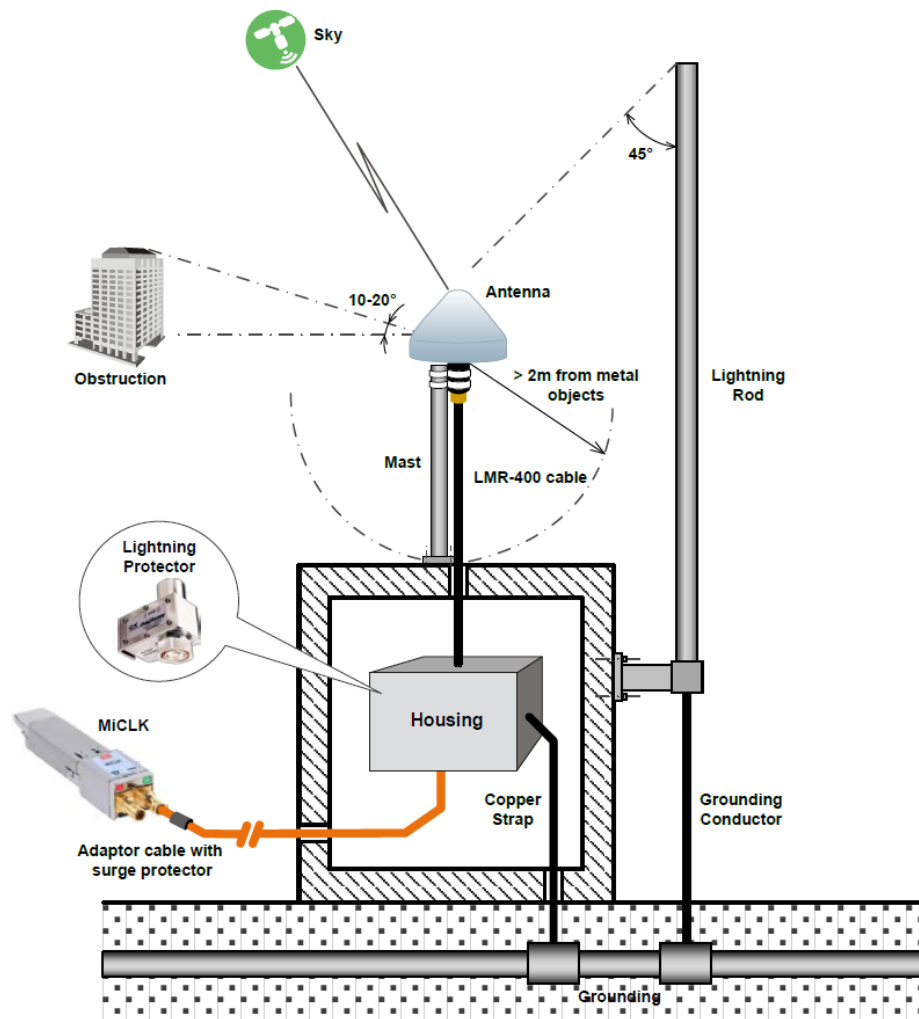
Figure 2. Outdoor Antenna Installation
