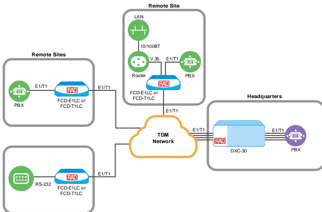
Figure 1. Extended Management over E1/T1 Network
