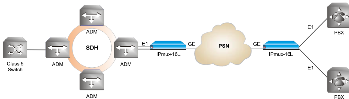
Figure 2. TDM Backhaul and Trunking over a PSN
