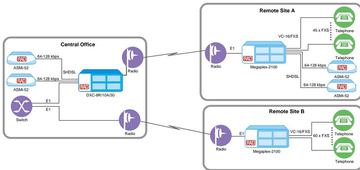
Figure 2. Voice and Data Extension
